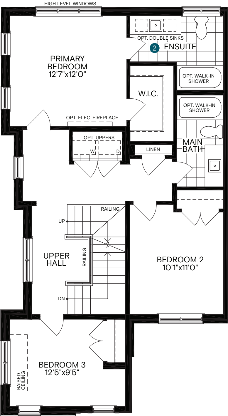
2ND FLOOR
