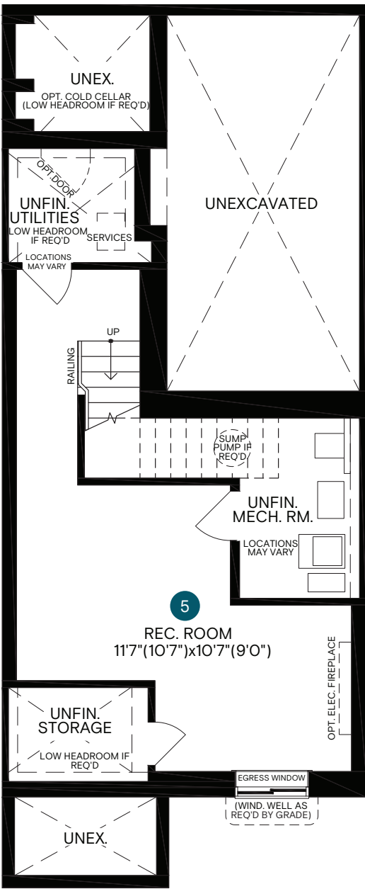
BASEMENT
